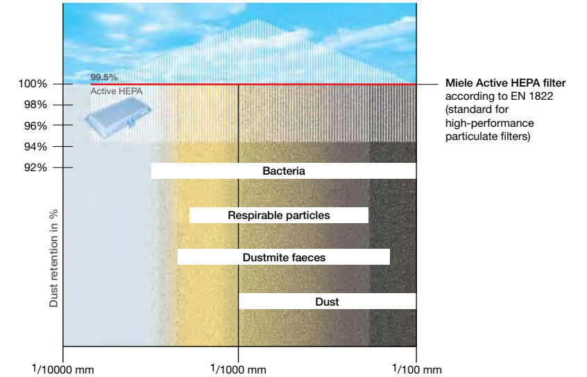
Dust retention performance of the Miele Active HEPA filter
